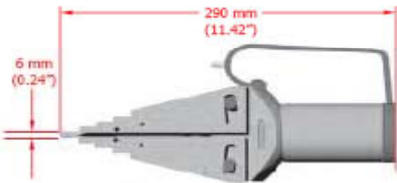
TOOL DIMENSIONS - CLOSED
